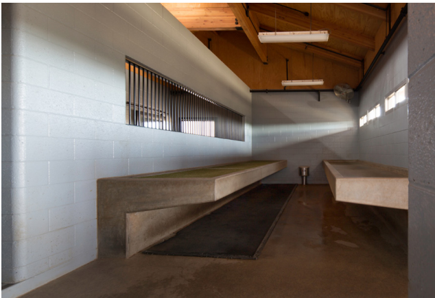
The cast-in-place concrete kennel beds incorporate heating systems and provide warm or cool bed options for the dogs.
